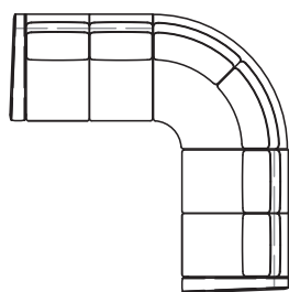
Motion: -55, -67, -56 Stationary: -57, -68, -58 Left Side: 108W Right Side: 108W 43 1/2D x 41H
