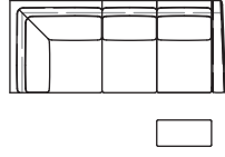
RAF Sofa Corner Return Recliner At Arm w/Power Headrest 201-74: 98W x 43 1/2D 202-74: 101W x 43 1/2D 203-74: 98W x 43 1/2D 204-74: 99W x 43 1/2D 206-74: 101W x 43 1/2D All: 41H
