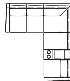
Motion: -73, -37, -07, -18 Left Side: 101W Right Side: 116W 43 1/2D x 41H
