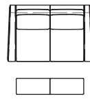
Loveseat L and R Full Recline w/Power Headrest 201-70: 61W x 43 1/2D 202-70: 67W x 43 1/2D 203-70: 61W x 43 1/2D 204-70: 64W x 43 1/2D 206-70: 67W x 43 1/2D All: 41H
