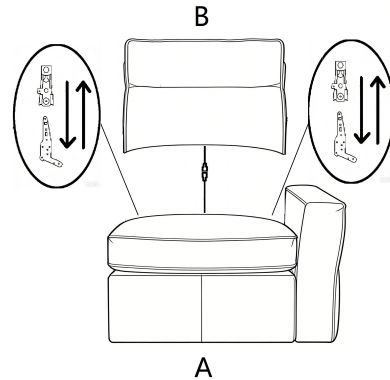
STEP 2 - Place Bracket into Sleeve and press top of back down firmly to lock your KD back in place
