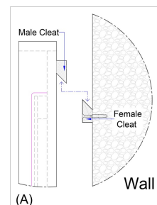
Side view of cleat engagement
