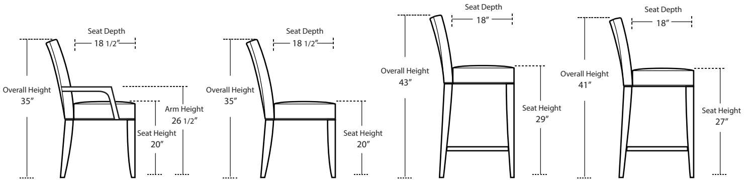
Arm Chair
