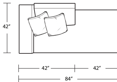
LAF 1 Arm Chair with Bumper
