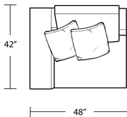
48" LAF 1 Arm Chair
