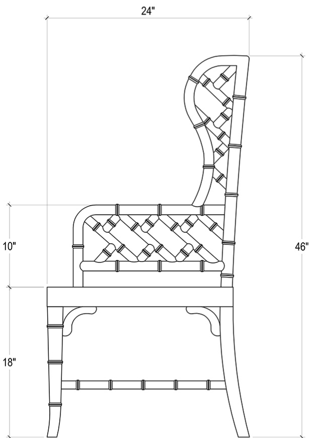
SIDE VIEW
