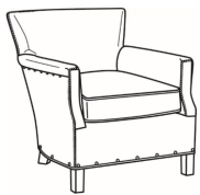
Francois / 1445 Chair (29W) Outside: 29W x 32D x 31H Inside: 19W x 20.5D
