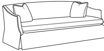
Braddock / 5450-00B Sofa (84W) Outside: 84W x 34D x 32.5H Inside: 76.5W x 21D
